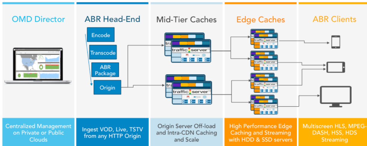
Figure 1. Synamedia Media Streamer Typical Deployment
